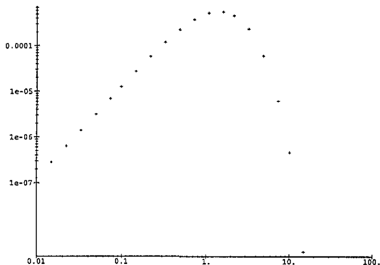
Figure 5. The difference (v_{L1})^2|_{Boltzmann} - (v_{L1})^2|_{Bose} as a function of \gamma = mc^2/kT . Note that the characteristic velocity for Boltzmann's gas is greater than for Bose's gas.
