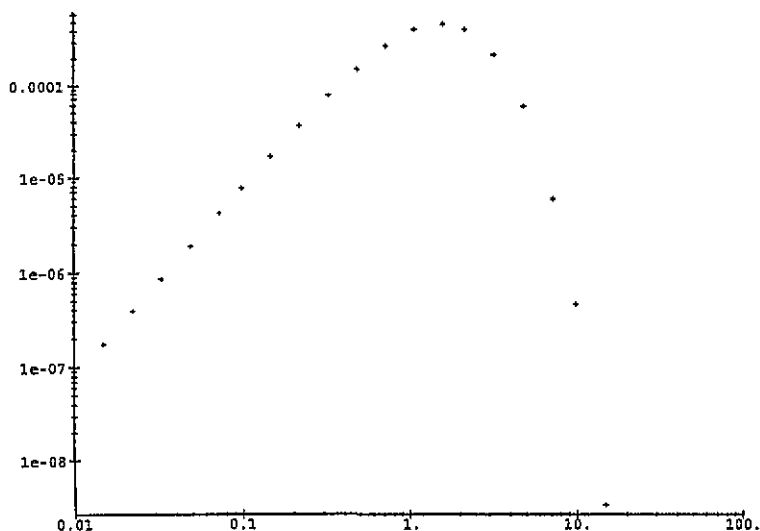
Figure 4. The difference (v_{L1})^2|_{Fermi} - (v_{L1})^2|_{Boltzmann} as a function of \gamma = mc^2/kT . Note that the characteristic velocity for Fermi's gas is greater than for Boltzmann's gas.
